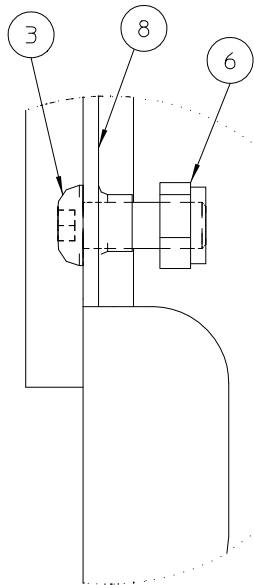
Detail1 SCALE 1:1
